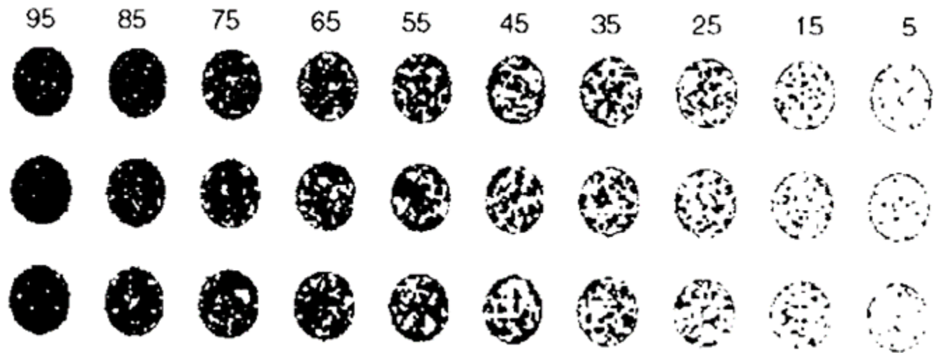
Guide for visually estimating cover. In this diagram black depicts cover, while white depicts open areas or bare ground.
