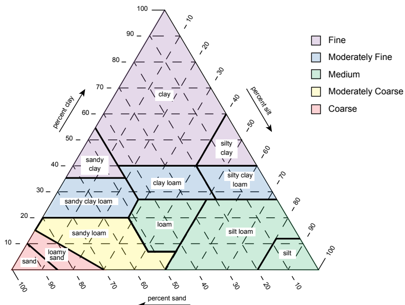
Figure 4. Chart showing the percent ages of clay, silt, and sand in the basic textural classes.
