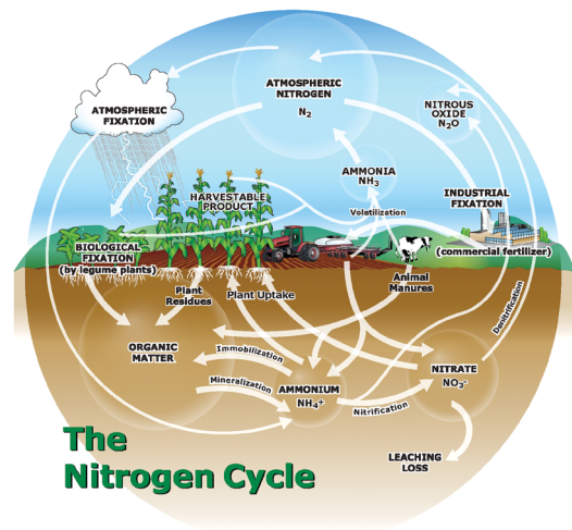
Figure 23.1 Important N transformations in agricultural soils. (Courtesy of IPNI)
