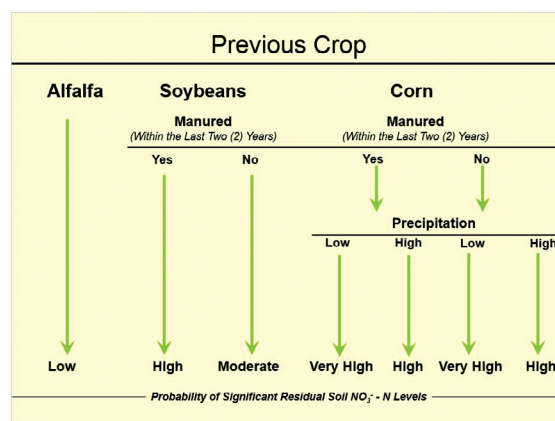
Figure 23.3 Probability of significant soil NO 3 -N level. (Reitsma et al., 2008)
