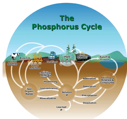
Figure 23.4 The phosphorus cycle. (Courtesy of International Plant Nutrition Institute)
